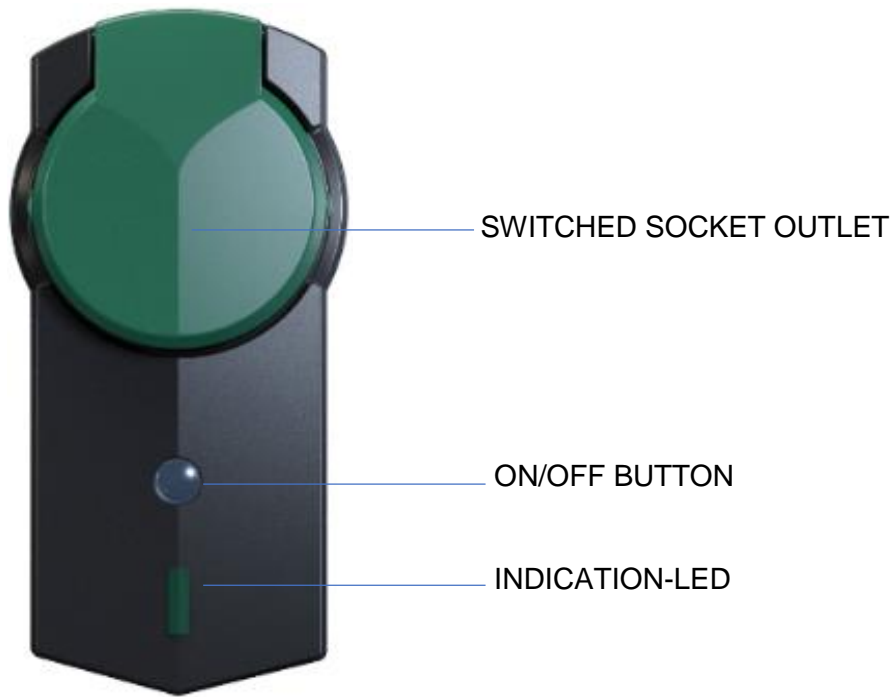
919.022 SMART Adapter
